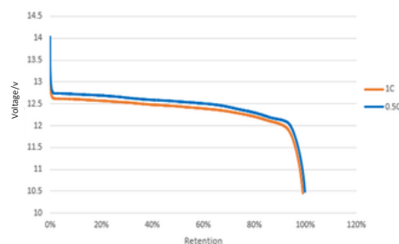
Discharge Curve at Different Rates @ 25°C
