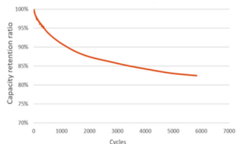
0.5C @ 80% DoD Cycle Life
