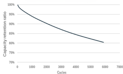
0.5C @ 80% DoD Cycle Life
