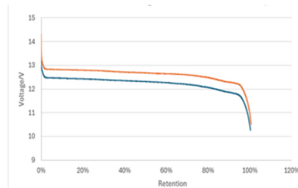
Discharge Curve at Different Rates @ 25°C
