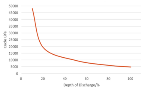
Cycle Life vs DoD @ 25°C
