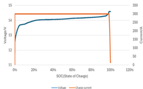
1C Charge Characteristics @ 25°C
